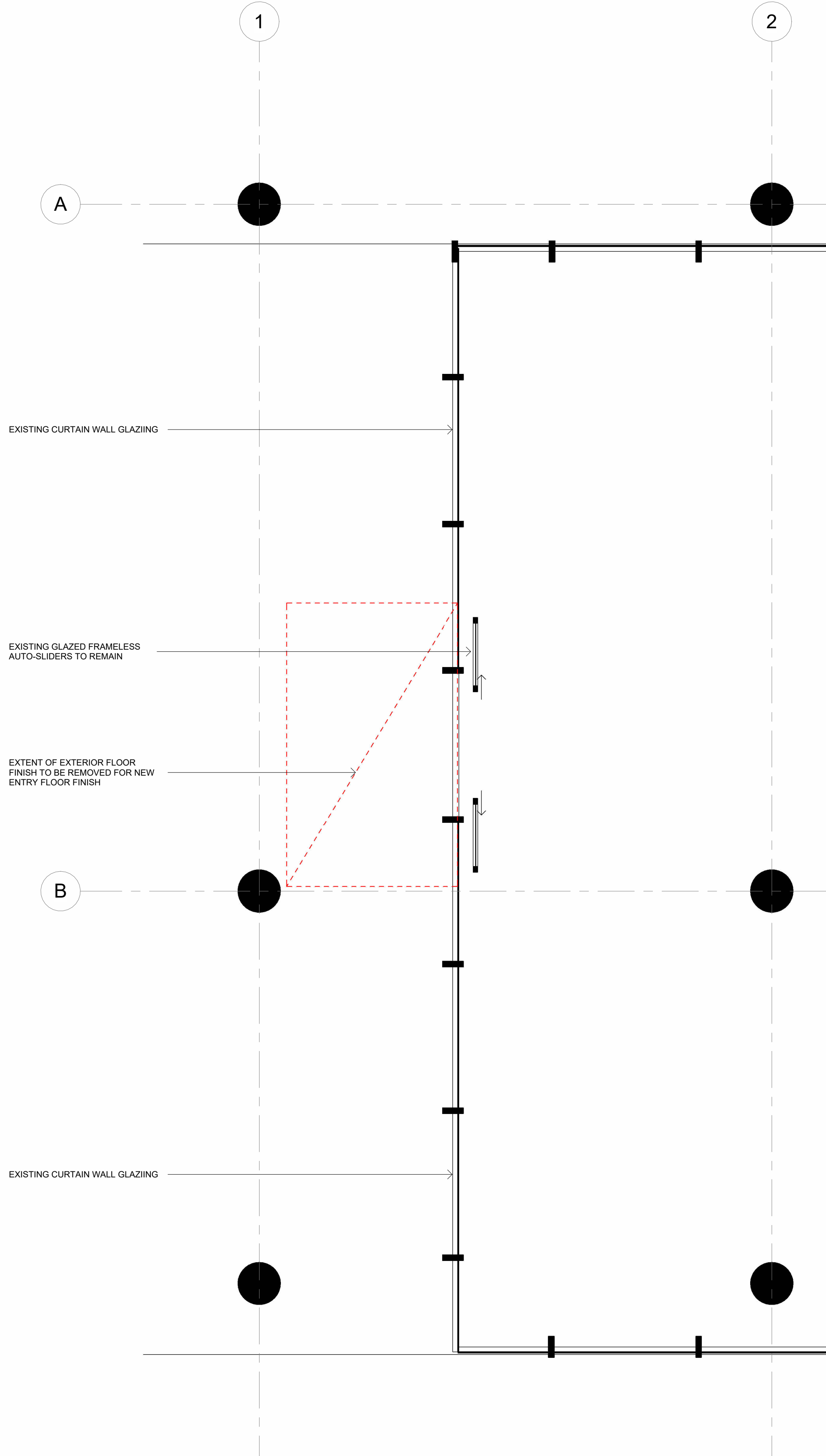
1 AIRLOCK DA DEMOLITION PLAN 1:50
